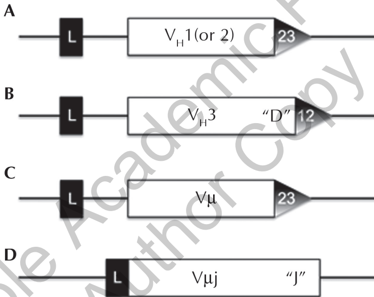
FIGURE 3 Diagram illustrating the basic structure of (A) a typical opossum germline V_H gene, (B) the partially germline joined opossum V_H 3 gene, (C) a typical opossum germline V_\mu gene, and (D) the germline joined opossum V_\mu j gene.
